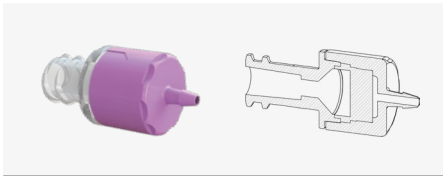
Check Valve | Female Luer Lock to 1/16" Barb
