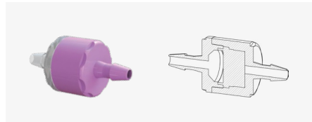
Check Valve | Male Luer 3/32" Barbs
