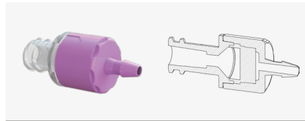
Check Valve | Female Luer Lock to 3/32" Barb
