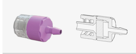
Check Valve | 3/32" Barb to Male Luer Lock
