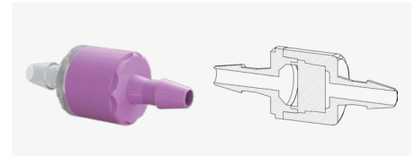
Check Valve | Male Luer 1/8" Barbs
